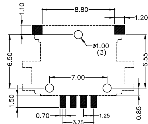
PCB LAYOUT
